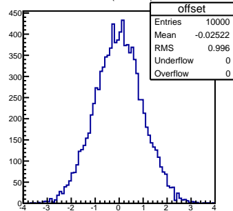
Offset: (fit-truth)/ \sigma
