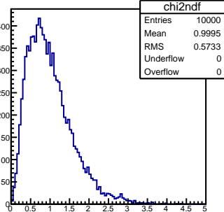
\chi^2/\text{ndf}
