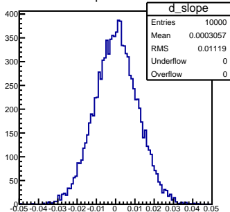
Slope: fit-truth
