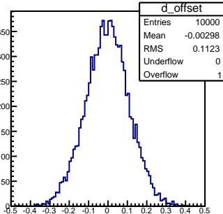
Offset: fit-truth
