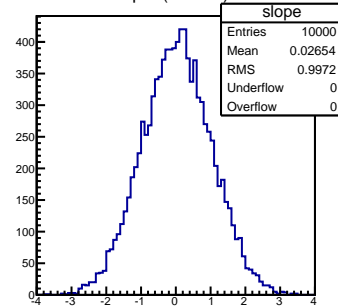
Slope: (fit-truth)/ \sigma
