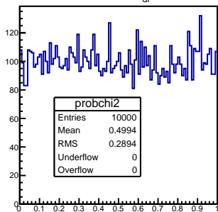
\text{Prob}(\chi^2, N_{\text{df}})
