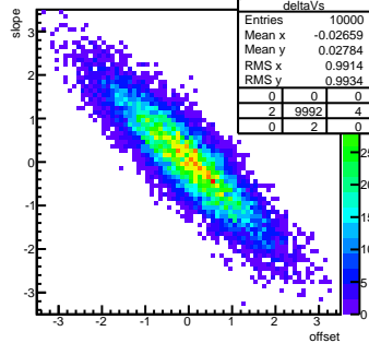
(\text{fit}-\text{true})/\sigma_{\text{fit}}
