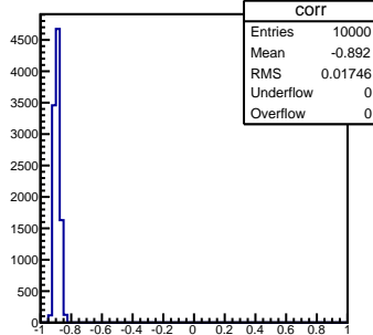
Correlation offset/slope
