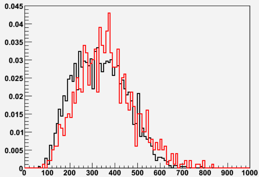
charged particle multiplicity
