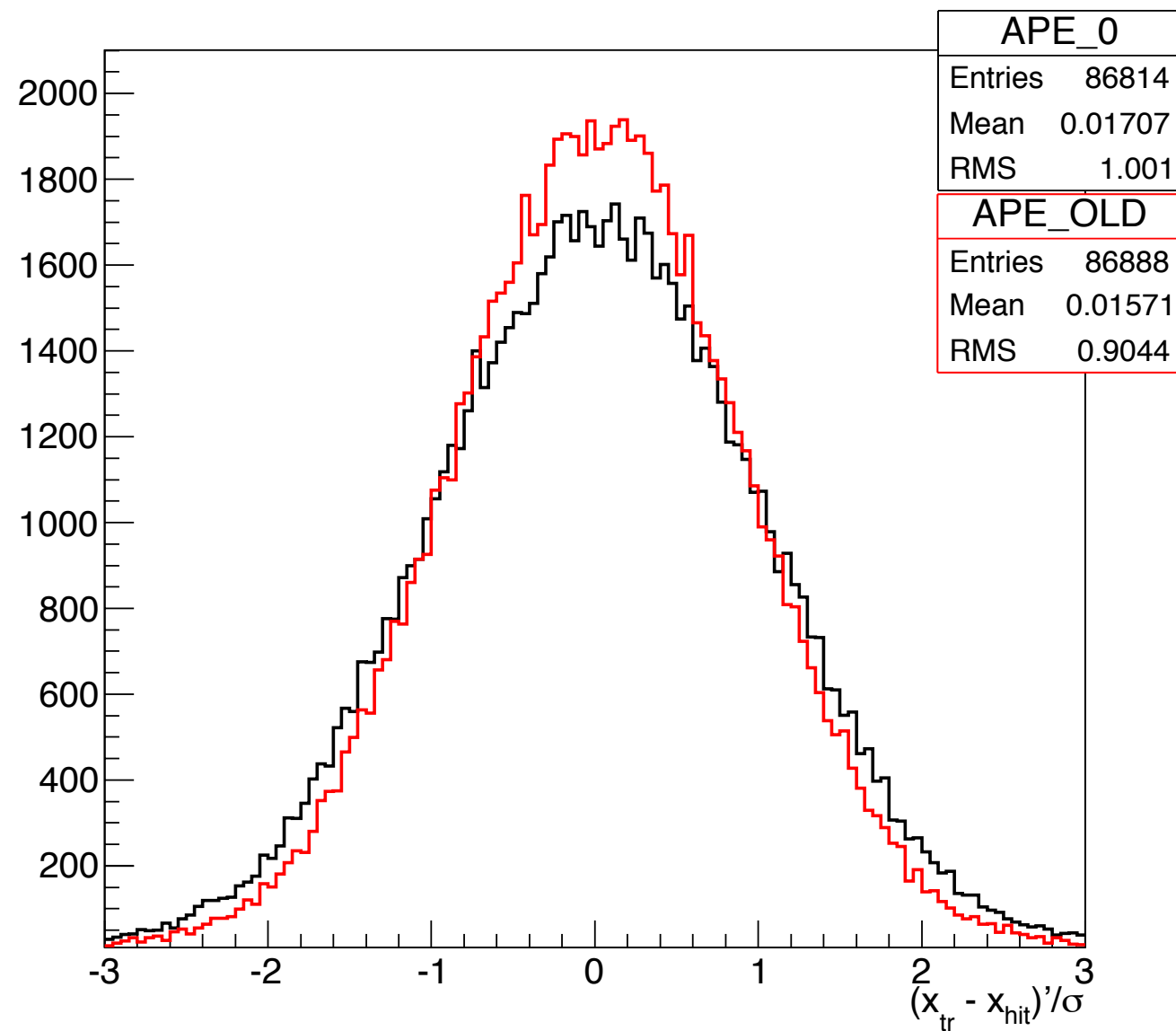
Residual for TPBBarrel 1 in Pixel
