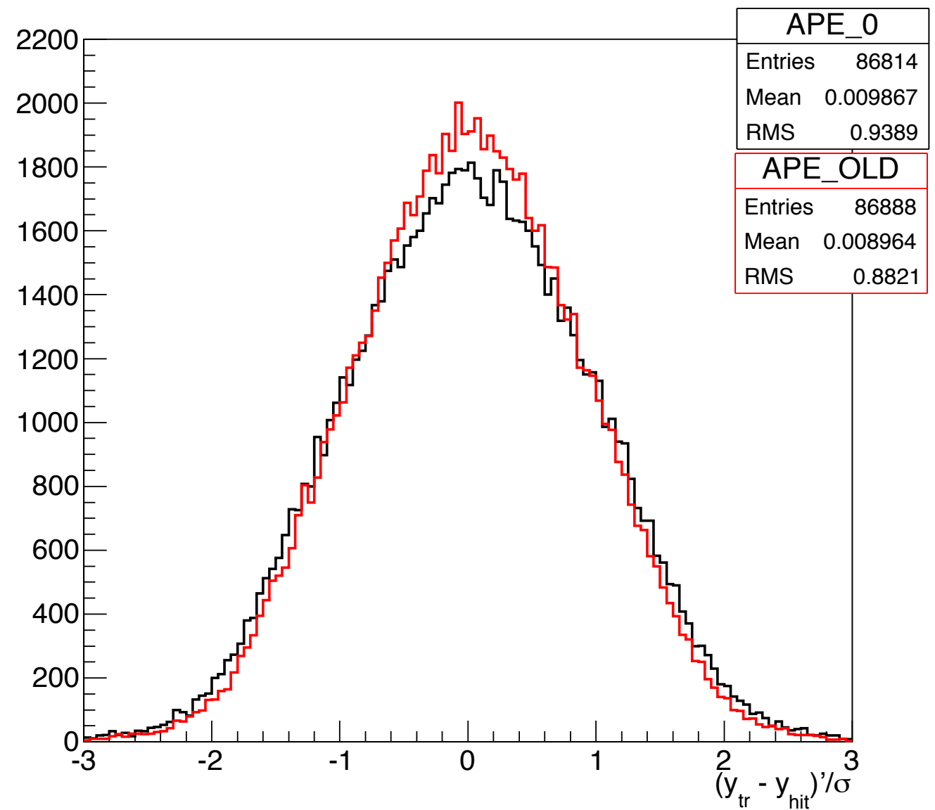
Residual for TPBBarrel 1 in Pixel
