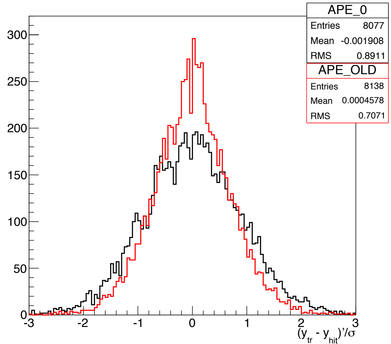
Residual for TPEEndcap 3 in Pixel
