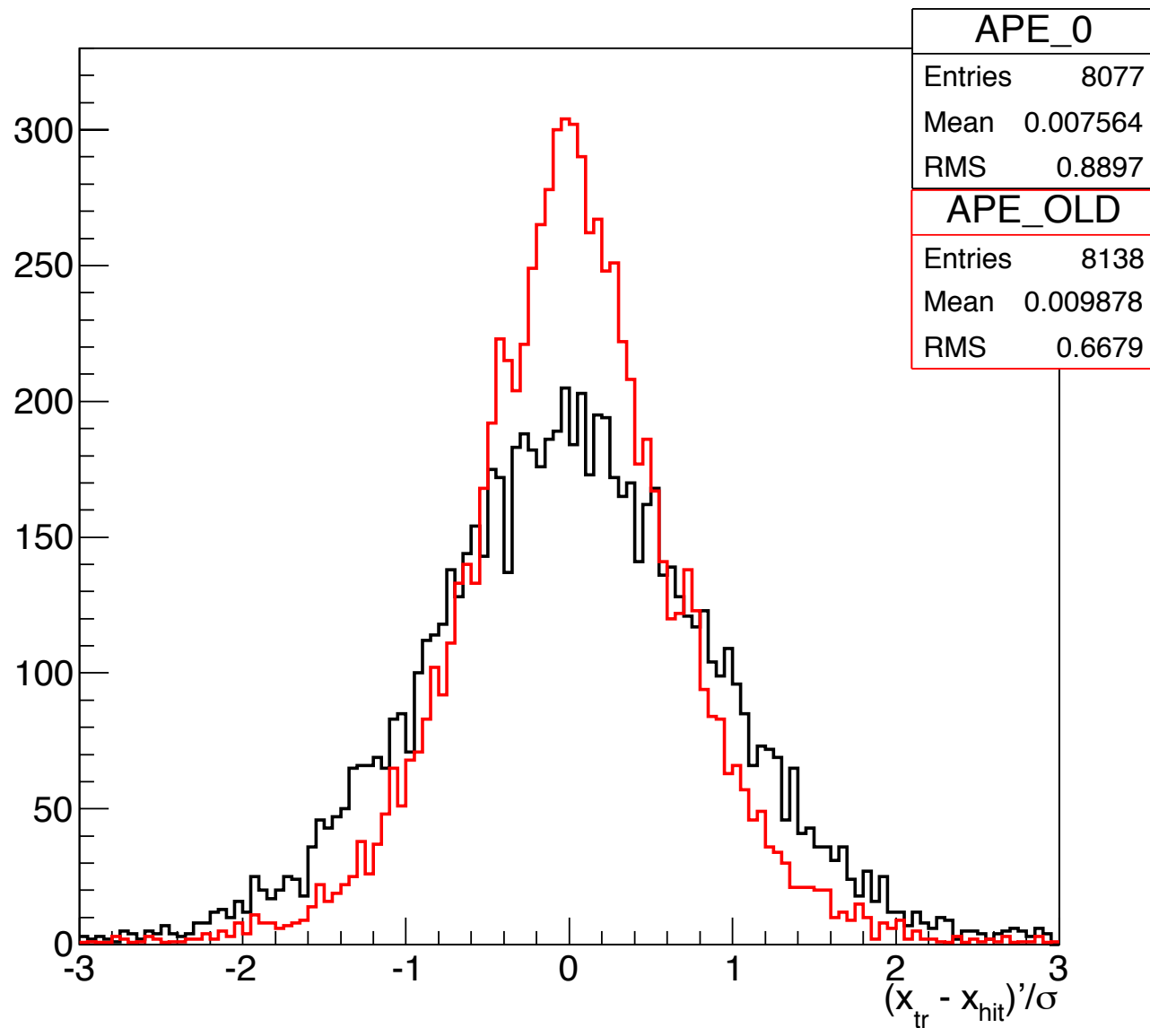
Residual for TPEEndcap 3 in Pixel
