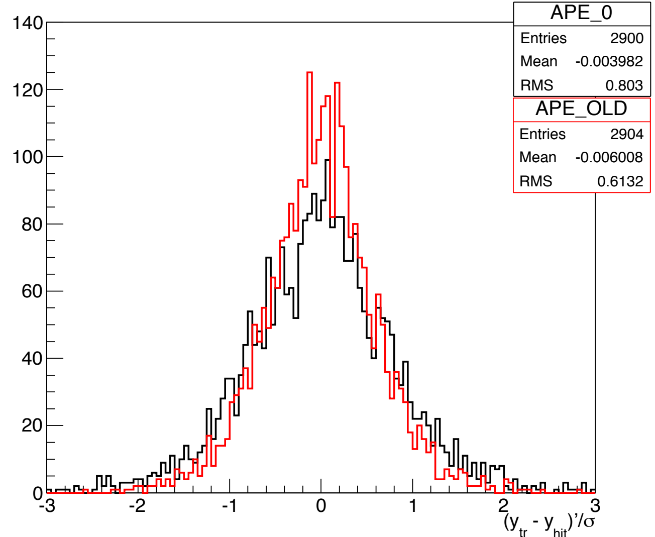
Residual for TPEEndcap 3 in Pixel
