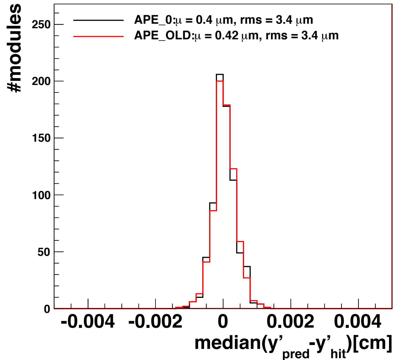
Distribution of the median of the y residuals in TPB
