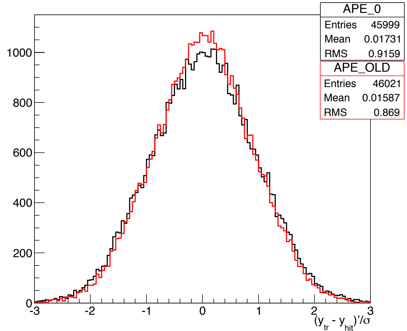
Residual for TPBBarrel 1 in Pixel
