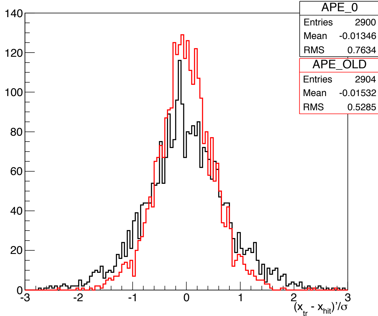
Residual for TPEEndcap 3 in Pixel
