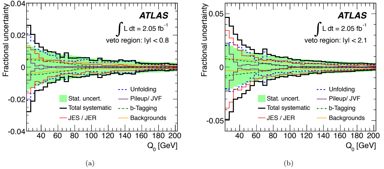
Fig. 3 Breakdown of the systematic uncertainties on the gap fraction as a function of Q_0 for (a) |y| < 0.8 and (b) |y| < 2.1 . The individual systematic uncertainties are shown as labelled lines of different styles and the total systematic uncertainty is shown as the outer solid line. The statistical uncertainty on the data is shown as the shaded area. The breakdown of the systematic uncertainties above Q_0 = 200 GeV is consistent with the results at Q_0 = 200 GeV. ‘Pileup’ refers to the effect of jets produced in a different proton-proton interaction. ‘Unfolding’ refers to the procedure used to correct the measured gap fraction to particle level.
