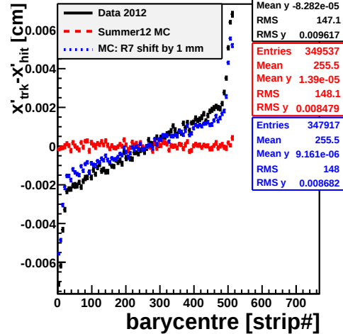
\Delta x' vs strip: W7
