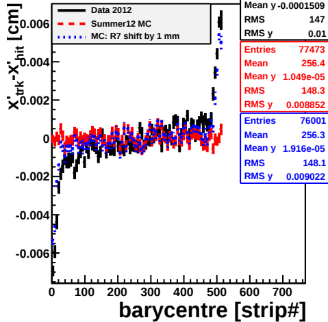
\Delta x' vs strip ( v_r > 0.5 ): W7
