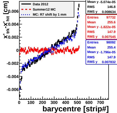
\Delta x' vs strip ( v_r < -0.5 ): W7
