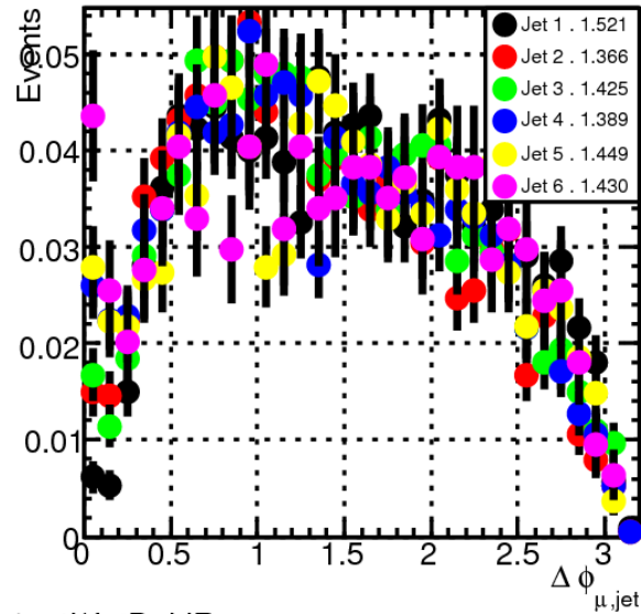
1m4j/JetDphiRec
