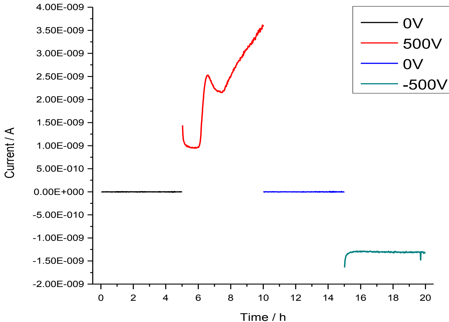
Current over Time for sc BCM1F Diamond +ZBottom
