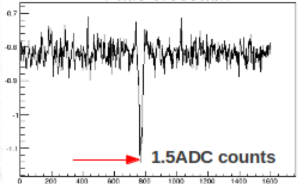
Pads crosstalk
