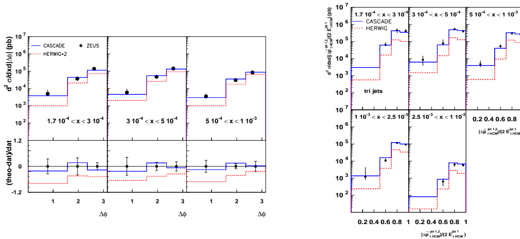
Fig. 4: (left) Angular correlations and (right) momentum correlations [18] in three-jet final states measured by [20], compared with k_{\perp} -shower (CASCADE) and collinear-shower (HERWIG) Monte Carlo results.
