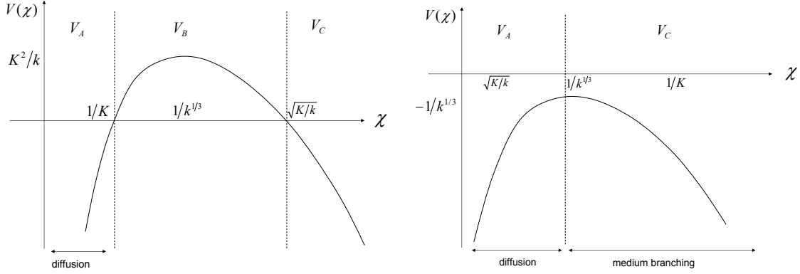
Fig. 1: The potential in the effective Schrödinger equation describing the propagation of the space-like Maxwell wave in AdS_5 -BH. Left: low energy, or large x ( x \gg T/Q ). Right: high energy, or small x ( x \lesssim T/Q )
