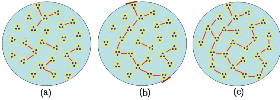
Fig. 3: (Color online) A schematic plot for the bond-percolation model. (a) Hadrons connected by bonds form clusters. (b) A cluster extending from one boundary to another is an infinite cluster. The appearance of infinite cluster is the start of crossover. (c) All the hadrons combined to a unique cluster is recognized as the end of crossover.
